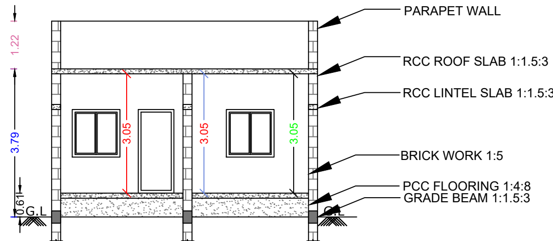
SECTION AB
