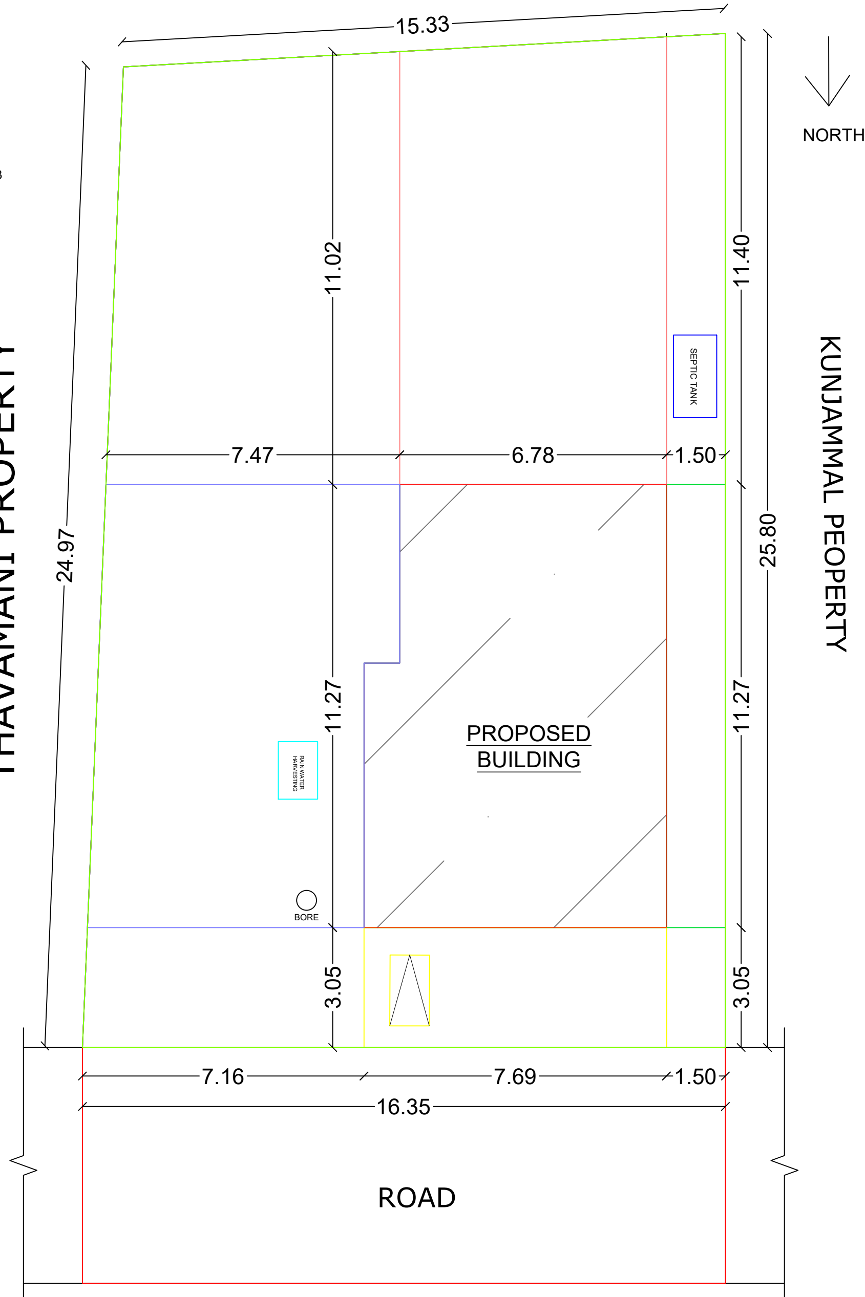
SITE PLAN
