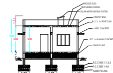
SECTION NO - "AA"
