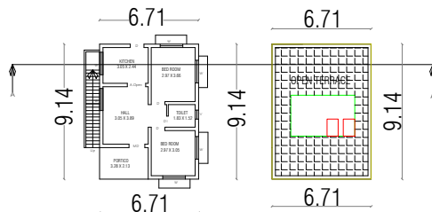
PRO.GROUND FLOOR PLAN
