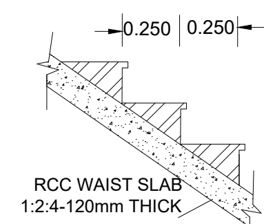
STAIR CASE STEPS SCALE 1:25
