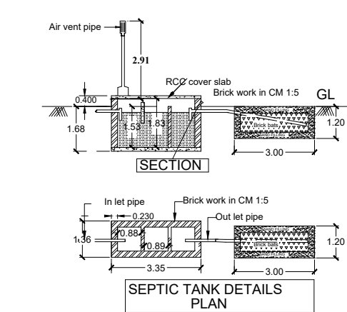
SEPTIC TANK DETAILS PLAN
