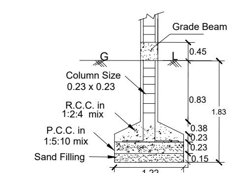
COLUMN DETAILS NOT TO SCALE
