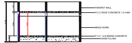
CROSS SECTION
