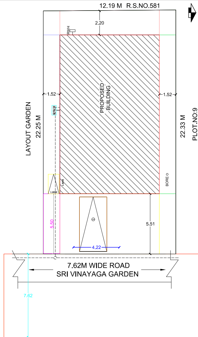
SITE PLAN
