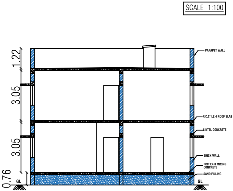
SECTION NO - "AB"
