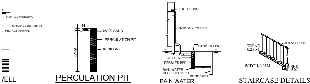
RAIN WATER
