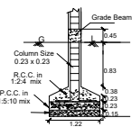
COLUMN DETAILS NOT TO SCALE
