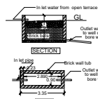
RAIN WATER HARVESTING TANK
