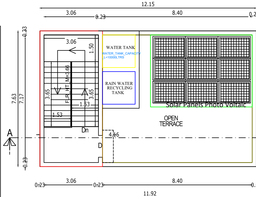
TERRACE PLAN
