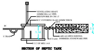
SECTION OF SEPTIC TANK
