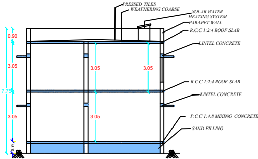
SECTION ON-AA
