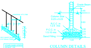
COLUMN DETAILS
