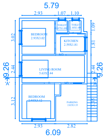
EXI-GROUND FLOOR PLAN
