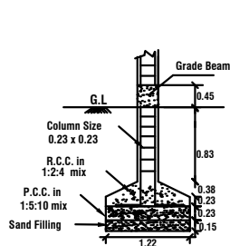
COLUMN DETAILS NOT TO SCALE
