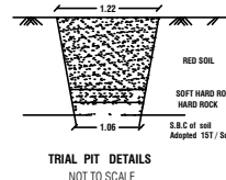
TRIAL PIT DETAILS NOT TO SCALE
