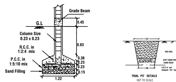
COLUMN DETAILS NOT TO SCALE
