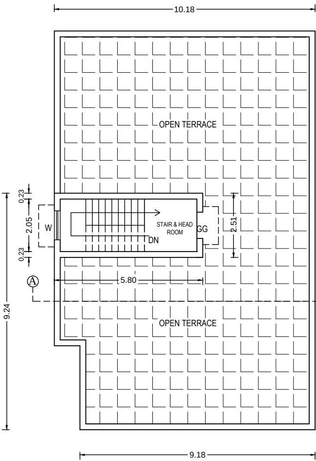
PRO - HEAD ROOM & OPEN TERRACE PLAN
