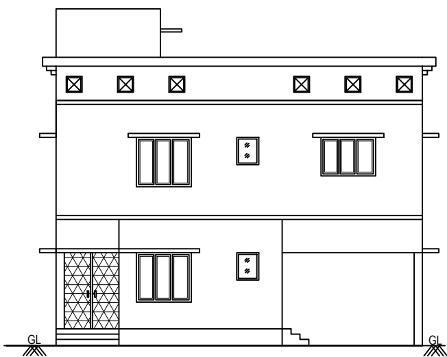
FRONT ELEVATION.
