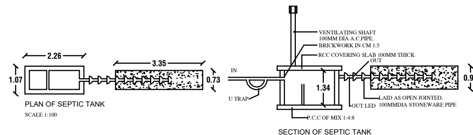
SECTION OF SEPTIC TANK
