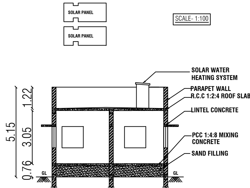
SECTION NO - "AB"
