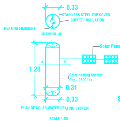
SCALE 1:50
