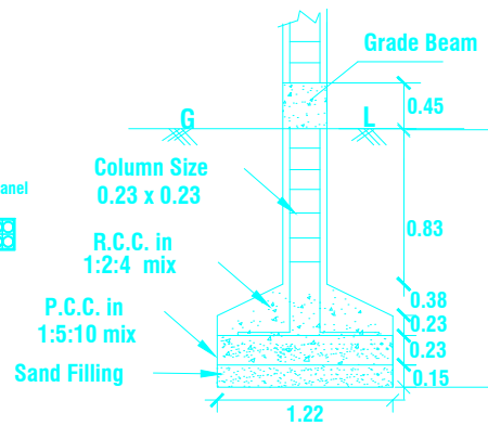
COLUMN DETAILS
