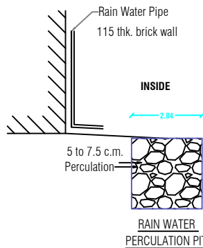
RAIN WATER PERCOLATION PIT
