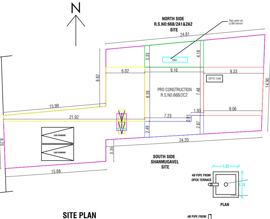
SCALE 1:50
