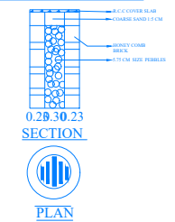
RAIN WATER HARVESTING L.PERCOLATION PIT
