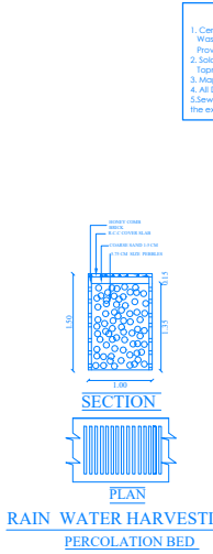
RAIN WATER HARVESTING PERCOLATION BED
