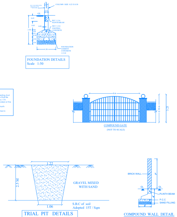
FOUNDATION DETAILS COMPOUND GATE TRIAL PIT DETAILS
