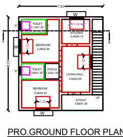
PRO.GROUND FLOOR PLAN
