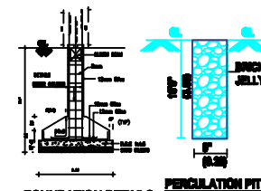
FOUNDATION DETAILS SCALE : 1:30
