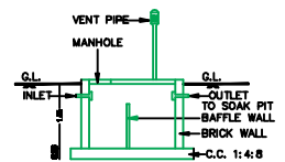
SECTION OF SEP. TANK
