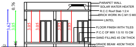
SECTION ON - AA
