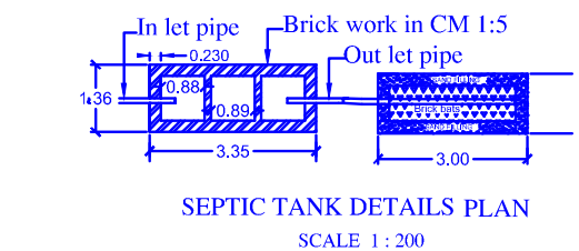
SEPTIC TANK DETAILS PLAN SCALE 1:200
