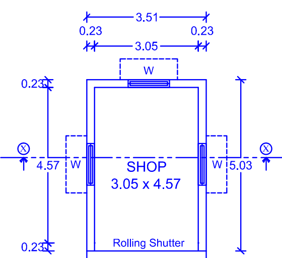
Ground Floor Plan Building No : 3
