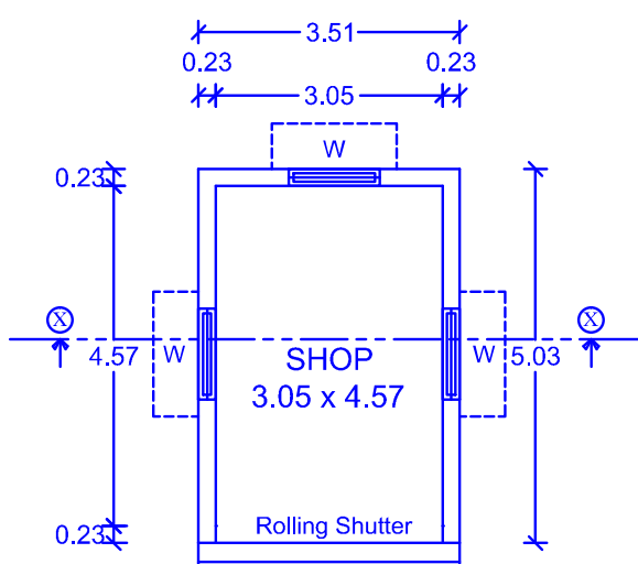
Ground Floor Plan Building No : 1
