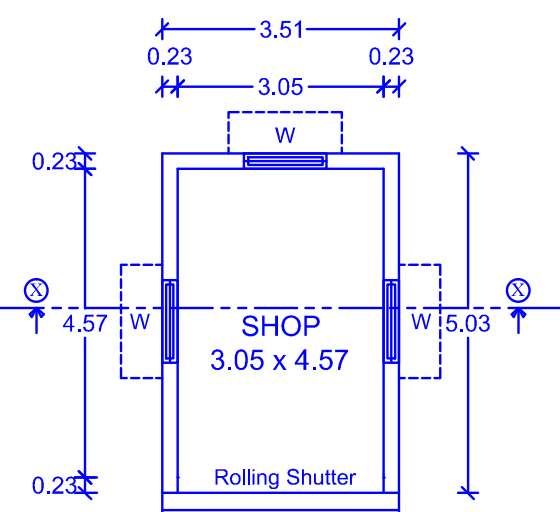
Ground Floor Plan Building No : 2
