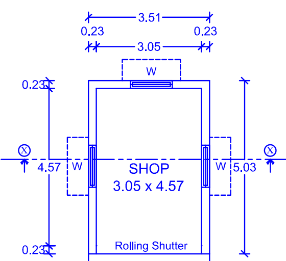
Ground Floor Plan Building No : 4
