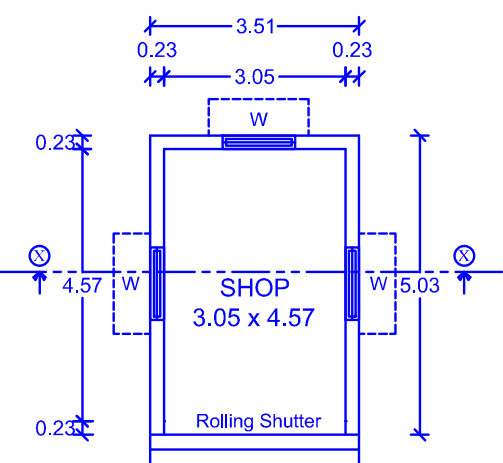
Ground Floor Plan Building No : 4
