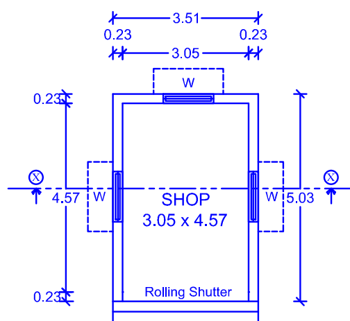
Ground Floor Plan Building No : 3
