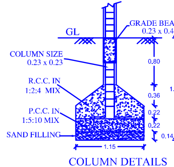
COLUMN DETAILS SCALE 1 : 50
