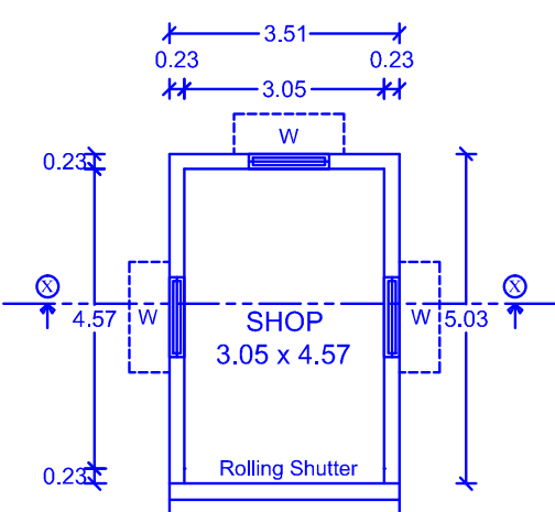
Ground Floor Plan Building No : 2
