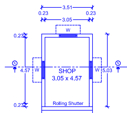
Ground Floor Plan Building No : 1
