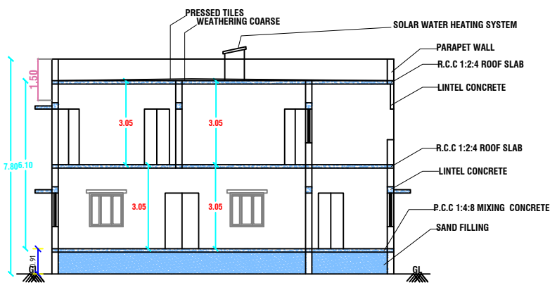
SECTION AT -'AA'
