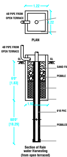
Section of Rain water Harvesting (from open terraced)
