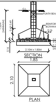
FOUNDATION DETAILS
