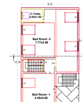
FLOOR PLAN
