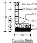
Foundation Details
