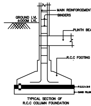
TYPICAL SECTION OF R.C.C. COLUMN FOUNDATION
