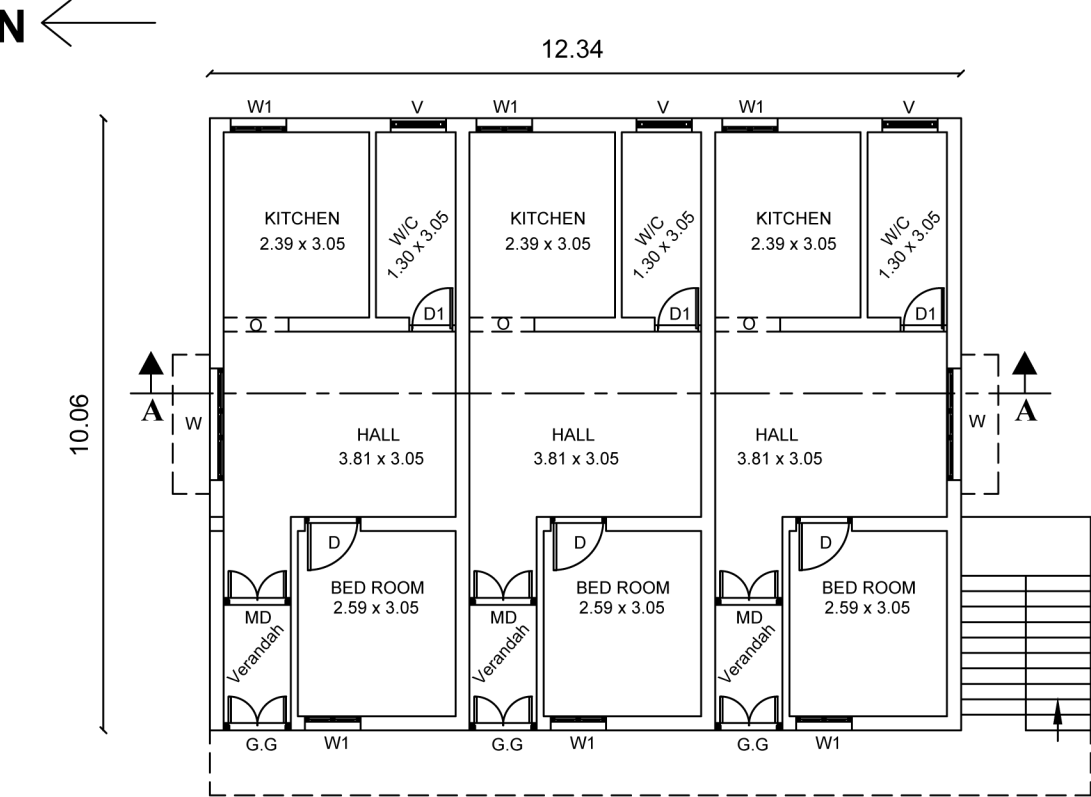
GROUND FLOOR PLAN BLOCK- 1
