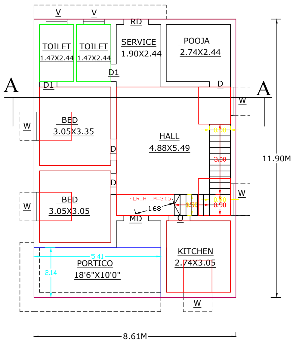
G.F. PLAN
