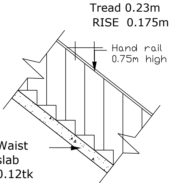
STAIRCASE
