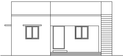
FRONT ELEVATION
