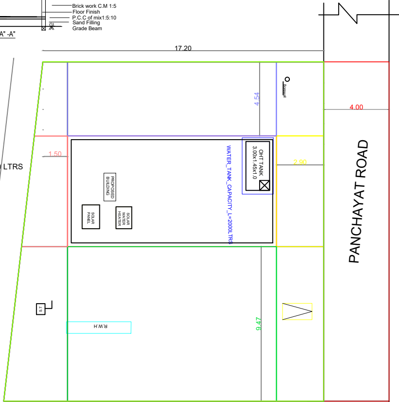
SCALE (1:100) SITE PLAN
