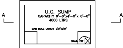
SUMP DETAIL SCALE 1"=4'0"
