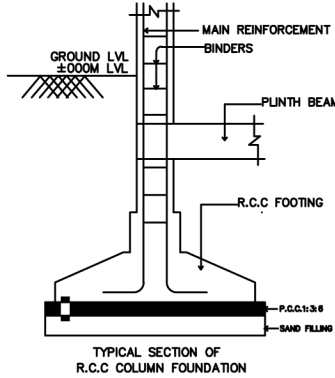
TYPICAL SECTION OF R.C.C COLUMN FOUNDATION
