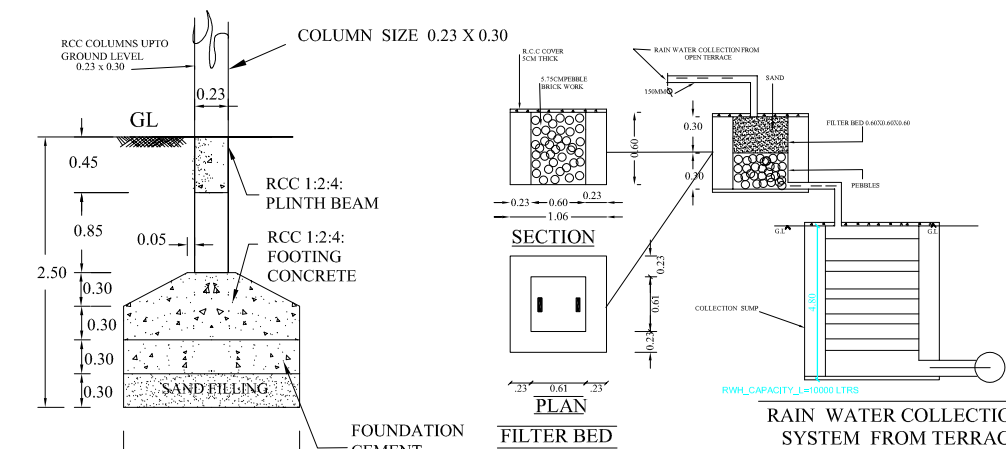
FOUNDATION DETAILS Scale 1:50
