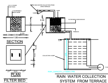
RAIN WATER HARVESTING PERCOLATION BED
