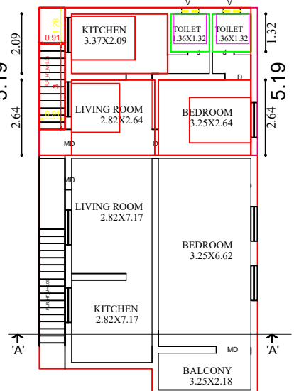
EXI.&PRO.FIRST FLOOR PLAN
