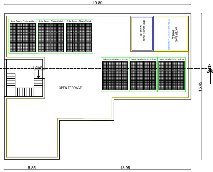
TERRACE PLAN
