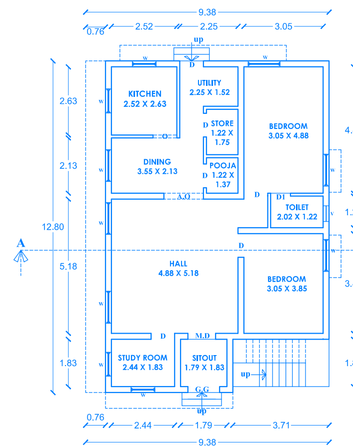
EXT. GROUND FLOOR PLAN
