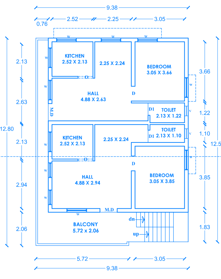
EXT. FIRST FLOOR PLAN
