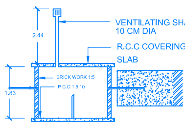
SEPTIC TANK DETAIL
