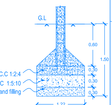
FOUNDATION DETAIL
