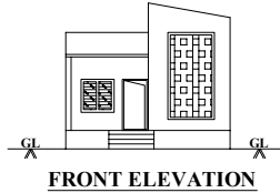
FRONT ELEVATION
