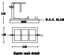
Septic tank detail
