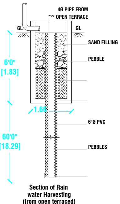
Section of Rain water Harvesting (from open terraced)
