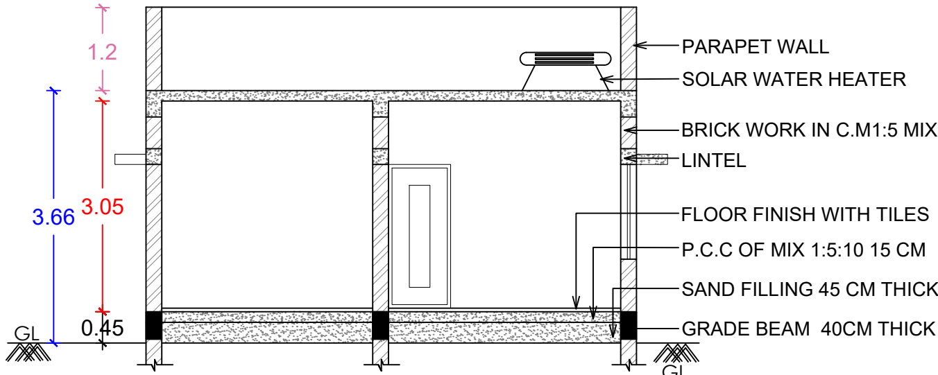
SECTION- AB
