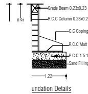
Foundation Detail
