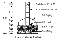
Foundation Detail
