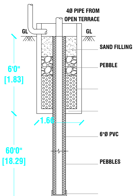
Section of Rain water Harvesting (from open terraced)
