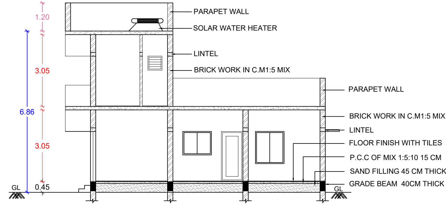
SECTION- AB
