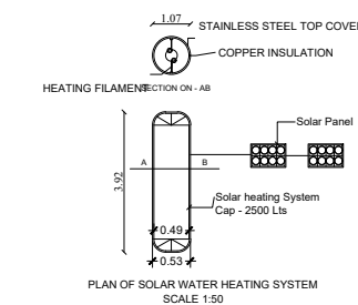
PLAN OF SOLAR WATER HEATING SYSTEM
