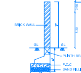
COMPOUND WALL DETAIL
