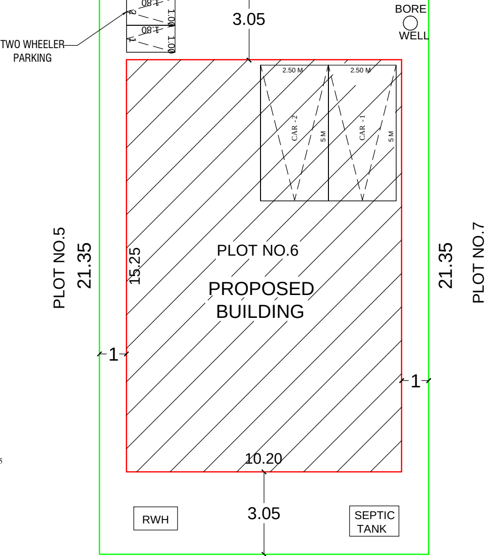
SITE PLAN
