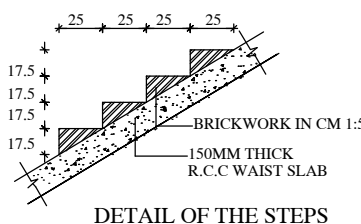
DETAIL OF THE STEPS
