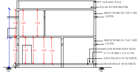
SECTION-AA1
