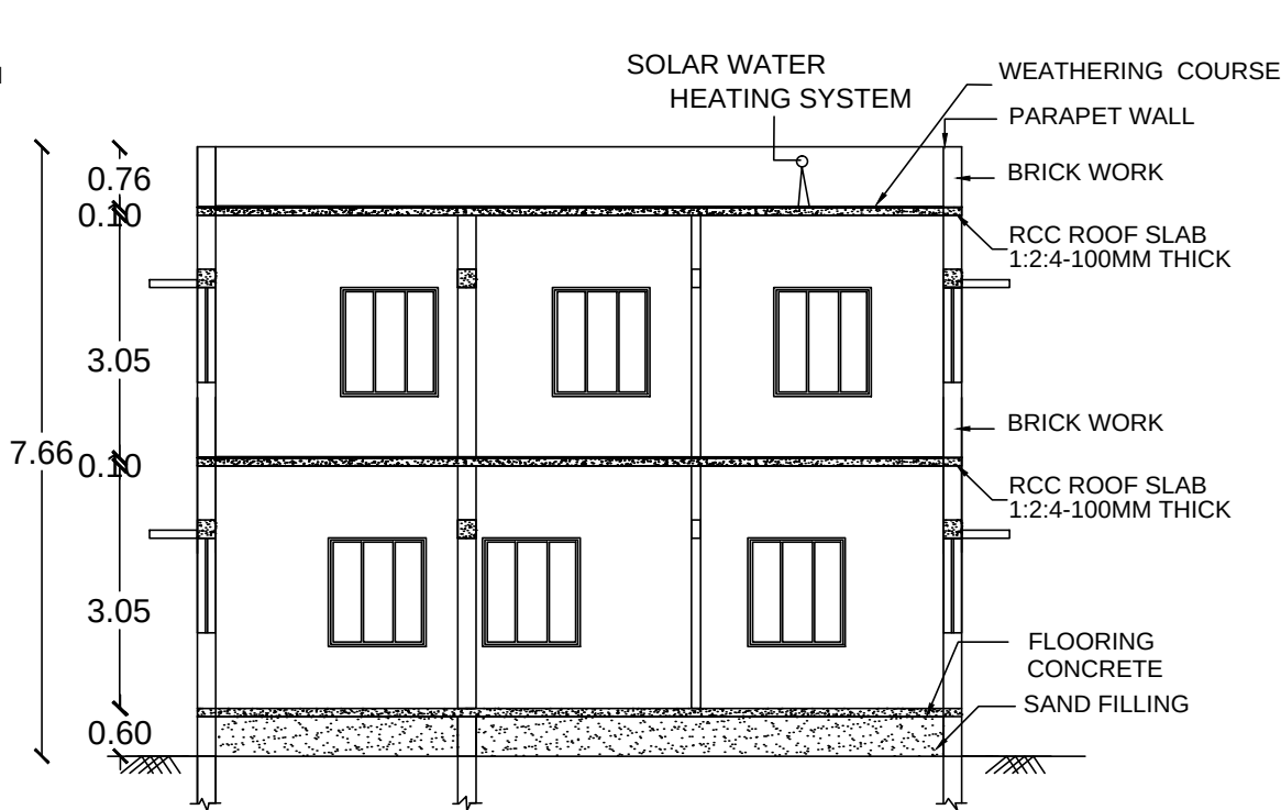
SECTION ON BR
