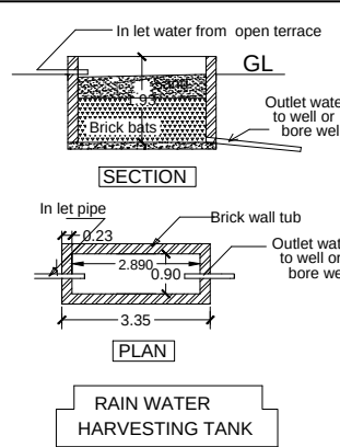
RAIN WATER HARVESTING TANK
