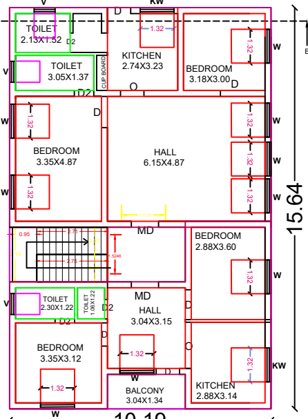
PRO.FIRST FLOOR
