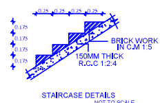
STAIRCASE DETAILS NOT TO SCALE
