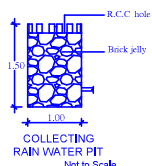
RAIN WATER PIT Not to Scale
