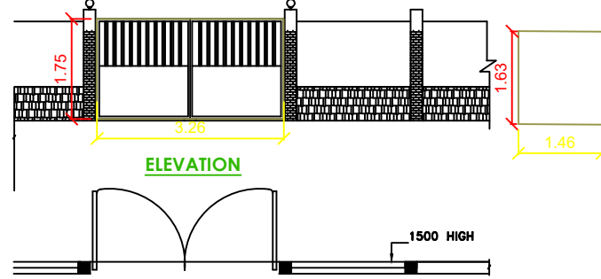
COMPOUND WALL DETAILS
