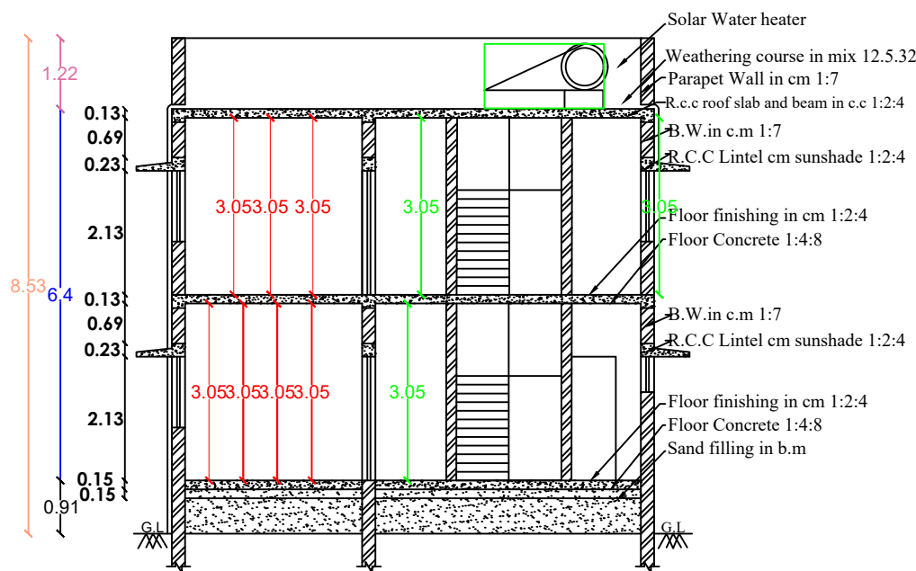
SECTION - "AB,AB"
