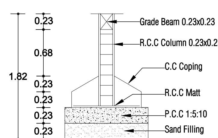
Foundation Detail
