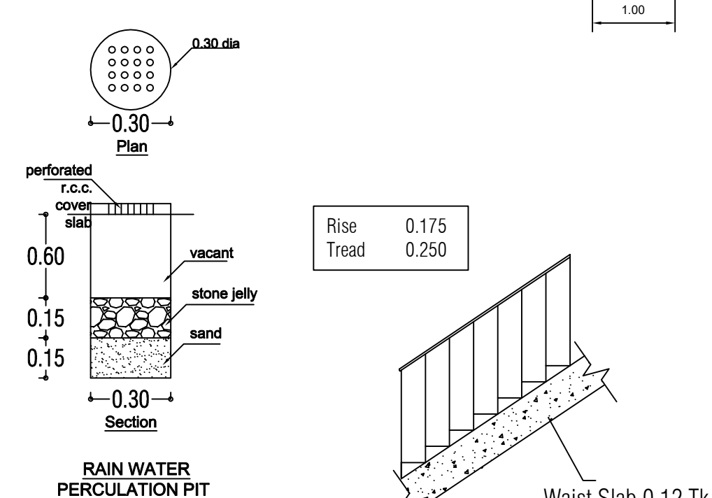
Staircase Details
