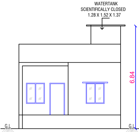
FRONT ELEVATION (PROPOSED)
