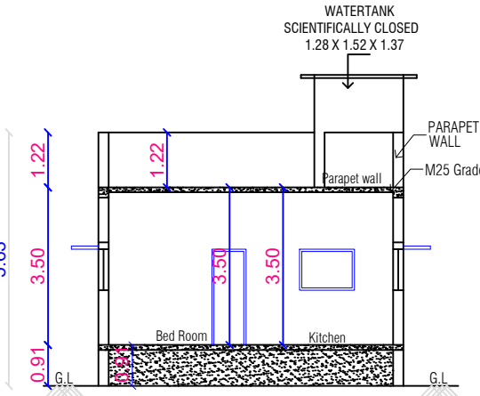
SECTION - AA (PROPOSED)
