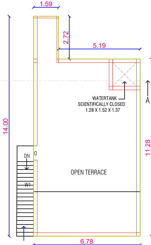
TERRACE FLOOR PLAN (PROPOSED)
