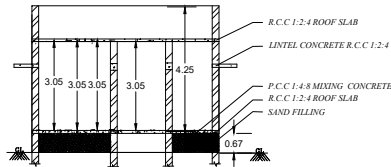
SECTION ON-'AB'
